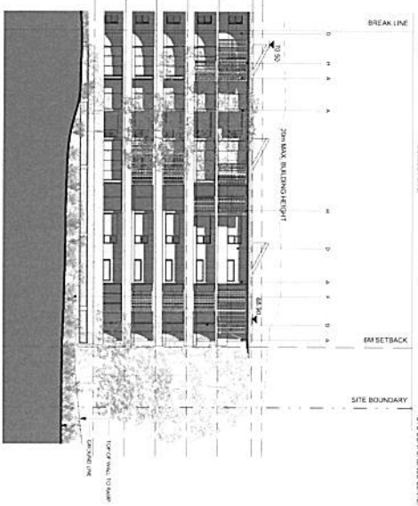
2 Building A Elevation West 1
