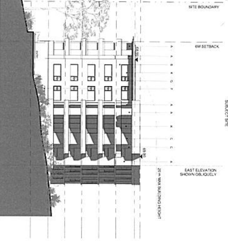
Building A - South Elevation
